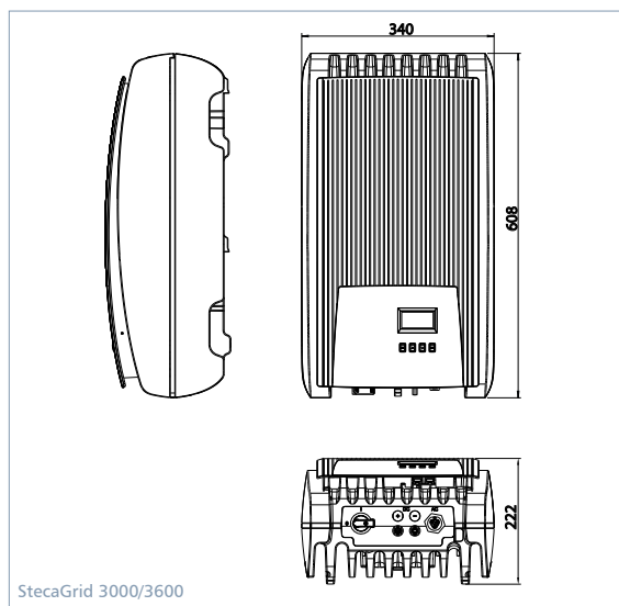
StecaGrid 3000/3600
